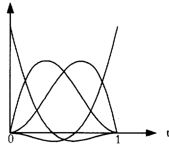
(Fig. 8) Generalized Bezier Basis 2
