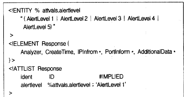
(Figure 9) DTD of response message
