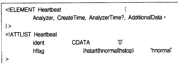
(Figure 7) DTD of modified heartbeat message
