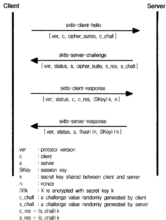
(Figure 12) The connection setup of SKTLS
