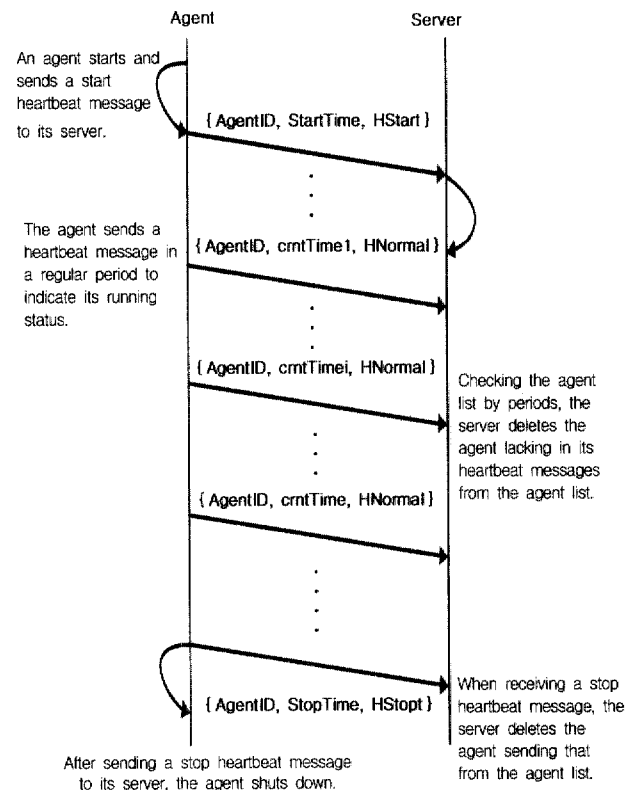
(Figure 5) Heartbeat message exchange procedure
