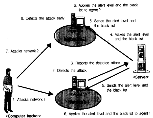
(Figure 1) Hierarchical detection processing of DS-NVSA
